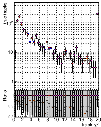
N of reco track vs. \chi^2 for B0M V0001, B0M V0002, B0M V0003, B0M V0004, B0M V0005, B0M V0006, B0M V0007, B0M V0008, B0M V0009, B0M V0010, B0M V0011, B0M V0012, B0M V0013, B0M V0014, B0M V0015, B0M V0016, B0M V0017, B0M V0018, B0M V0019, B0M V0020, Global fit 10000, RECO
