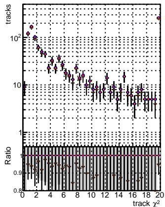
N of reco track vs. \chi^2 for B0M V0001, B0M V0002, B0M V0003, B0M V0004, B0M V0005, B0M V0006, B0M V0007, B0M V0008, B0M V0009, B0M V0010, B0M V0011, B0M V0012, B0M V0013, B0M V0014, B0M V0015, B0M V0016, B0M V0017, B0M V0018, B0M V0019, B0M V0020, Global fit 10000, RECO
