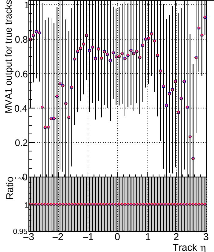
MVA1 of associated tracks (recoToSim) vs. track \eta DOM V0001 R000000001 Global mkFit1000o RECO DOM V0001 R000000001 Global mkFit1000 RECO DOM V0001 R000000001 Global mkFit1000ATime RECO DOM V0001 R000000001 Global mkFit1000CTime RECO DOM V0001 R000000001 Global mkFit1000MTIME RECO
