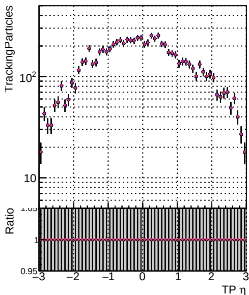
N of sim DOM V0001 R0000000001 Global mkFit10000 RECO DOM V0001 R0000000001 Global mkFit10000 RECO DOM V0001 R0000000001 Global mkFit10000 RECO DOM V0001 R0000000001 Global mkFit1000ATime RECO DOM V0001 R0000000001 Global mkFit1000CTime RECO DOM V0001 R0000000001 Global mkFit1000MTime RECO
