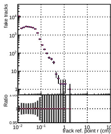
N of fake tracks vs transverse ref point position
