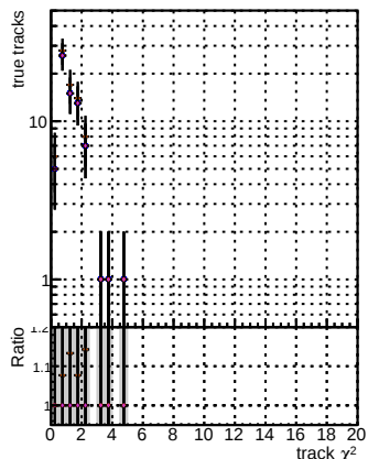
N of reco track vs. \chi^2 Global fit 10000 RECO BGM V0001 B0000000001 Global fit 10000 RECO BGM V0001 B0000000001 Global fit 10000 RECO
