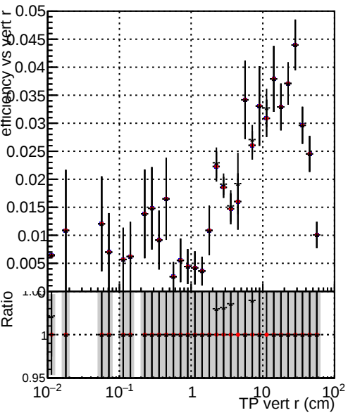
Efficiency vs TP vert r (cm) Legend: DQM_V0001_R0000000001_Global_mkFit1000o_RECO DQM_V0001_R0000000001_Global_mkFit1000_RECO DQM_V0001_R0000000001_Global_mkFit1000ATime_RECO
