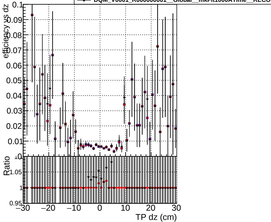
Efficiency vs Dz
