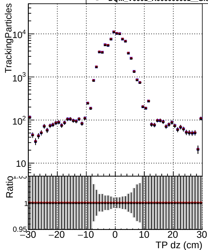
N of simulated tracks vs TP dz (cm) Legend: DQM_V0001_R000000001_Global_mkFit1000o_RECO DQM_V0001_R000000001_Global_mkFit1000_RECO DQM_V0001_R000000001_Global_mkFit1000ATime_RECO
