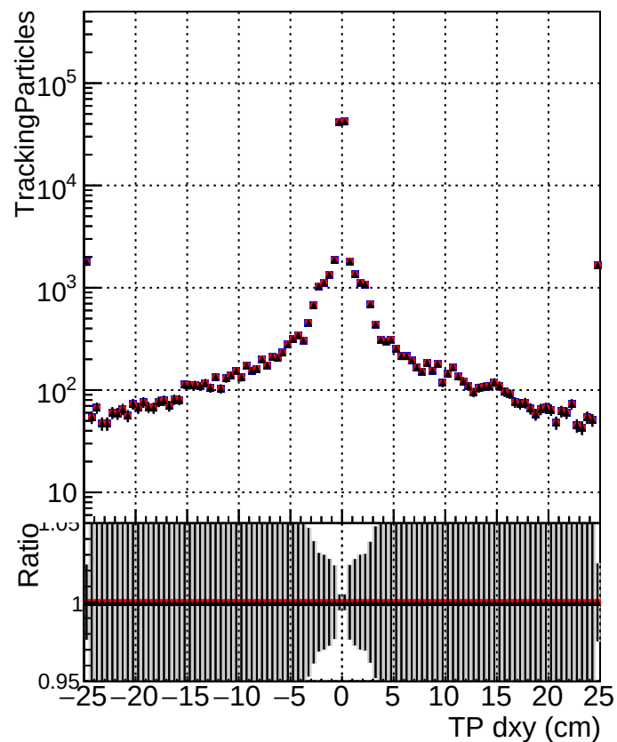
N of simulated track ■ DQM_V0001_R000000001 Global mkFit1000o RECO ● DQM_V0001_R000000001 Global mkFit1000 RECO ▲ DQM_V0001_R000000001 Global mkFit1000ATime RECO
