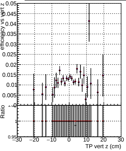
Efficiency vs TP vert z (cm) Legend: DQM_V0001_R0000000001_Global_mkFit1000o_RECO DQM_V0001_R0000000001_Global_mkFit1000_RECO DQM_V0001_R0000000001_Global_mkFit1000ATime_RECO
