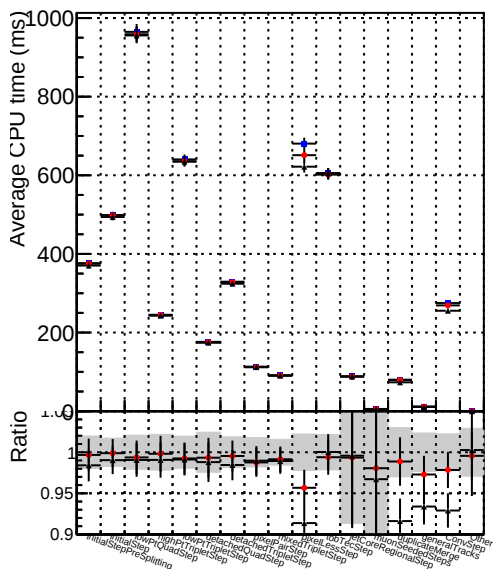
Average CPU time / event
