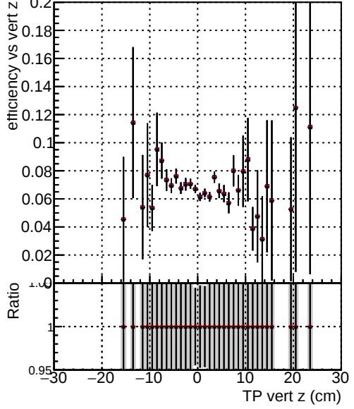
Efficiency vs vert z —●— DQM_V0001_R0000000001_Global_mkFit1000o_RECO —●— DQM_V0001_R0000000001_Global_mkFit1000_RECO —●— DQM_V0001_R0000000001_Global_mkFit1000ATime_RECO
