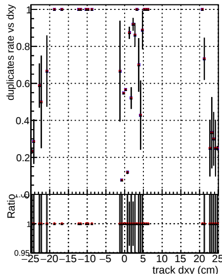
DOM V0001 RECO DOM V0001 RECO Global mkFit10000 RECO Global mkFit10000 RECO Global mkFit10000 RECO
