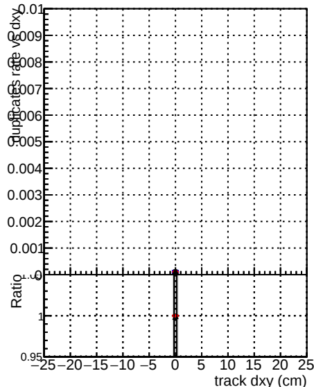
Legend for Fake rate vs dz, Duplicates Rate vs Dxy, and Pileup rate vs dz: DOM V0001 R0000000001 Global mkFit10000 RECO DOM V0001 R0000000001 Global mkFit10000 RECO DOM V0001 R0000000001 Global mkFit10000 RECO
