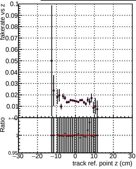
Legend: - DQM_V0001_R0000000001 Global mkFit1000o RECO - DQM_V0001_R0000000001 Global mkFit1000 RECO - DQM_V0001_R0000000001 Global mkFit1000ATime RECO
