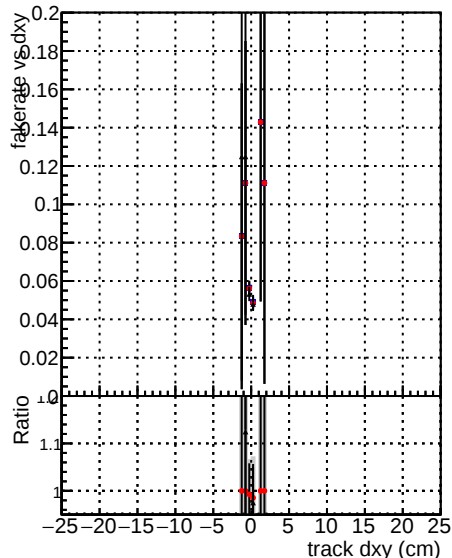
— DOM V0001 R0000000001 Global mkFit10000 RECO — DOM V0001 R0000000001 Global mkFit10000 RECO — DOM V0001 R0000000001 Global mkFit10000 RECO
