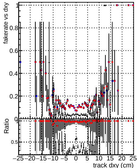
Legend for all plots: Global (black line) mkFit10000 (blue line) RECO (red line) Global (black line) mkFit1000 (blue line) RECO (red line) Global (black line) mkFit1000 (blue line) RECO (red line)
