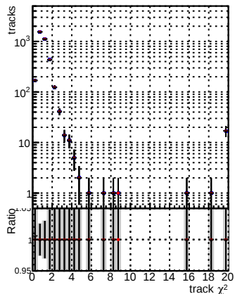
N of reco track vs. Global mktFit10000 RECO
