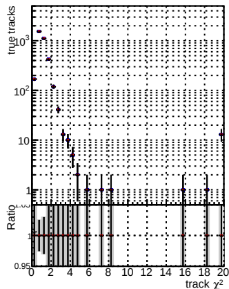
N of reco track vs. Global mktFit10000 RECO
