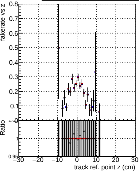
Legend: - Global mkFit1000o RECO - Global mkFit1000 RECO - Global mkFit1000ATime RECO
