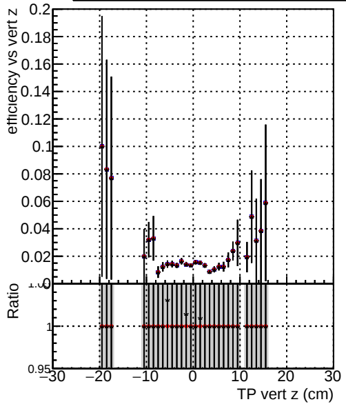
Efficiency vs. sim PV z —●— DQM_V0001_R0000000001_Global_mkFit1000o_RECO —●— DQM_V0001_R0000000001_Global_mkFit1000o_RECO —●— DQM_V0001_R0000000001_Global_mkFit1000ATime_RECO
