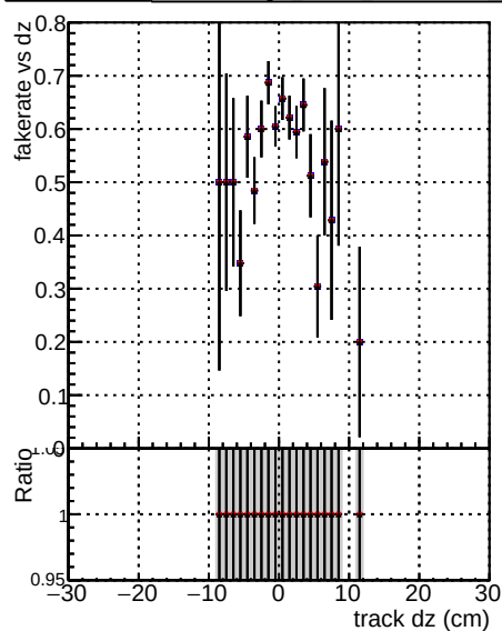
Fake rate vs dz Legend: DOM V0001 R0000000001 Global mkFit10000 RECO DOM V0001 R0000000001 Global mkFit10000 RECO DOM V0001 R0000000001 Global mkFit10000 RECO
