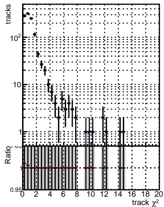
N of reco track vs. s DQM V0001 R000000000001 Global mkFit10000 RECO DQM V0001 R000000000001 Global mkFit10000 RECO DQM V0001 R000000000001 Global mkFit10000 RECO DQM V0001 R000000000001 Global mkFit10000 RECO
