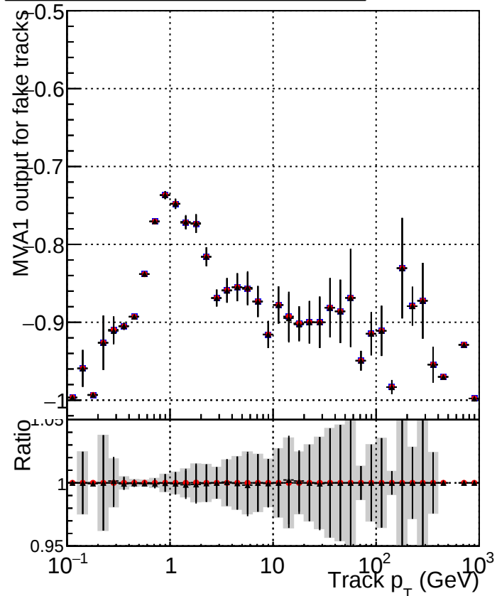
MVA1 of associated tracks (recoToSim) vs. track \eta Legend: DQM_V0001_R000000001_Global_mkFit1000o_RECO DQM_V0001_R000000001_Global_mkFit1000_RECO DQM_V0001_R000000001_Global_mkFit1000ATime_RECO
