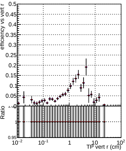
Efficiency vs vertpos DQM_V0001_R000000001_Global_mkFit1000o_RECO DQM_V0001_R000000001_Global_mkFit1000_RECO DQM_V0001_R000000001_Global_mkFit1000ATime_RECO
