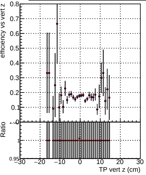
Efficiency vs vertpos Legend: DQM_V0001_R0000000001_Global_mkFit1000o_RECO DQM_V0001_R0000000001_Global_mkFit1000_RECO DQM_V0001_R0000000001_Global_mkFit1000ATime_RECO
