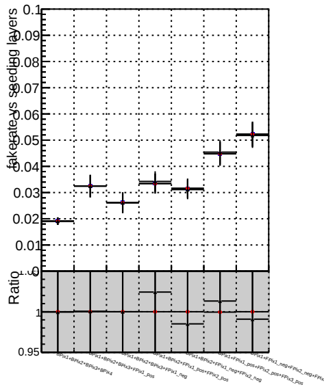
Fake rate vs. — DOM_V0001_R0000000001_Global_mkFit1000o_RECO — DOM_V0001_R0000000001_Global_mkFit1000o_RECO — DOM_V0001_R0000000001_Global_mkFit1000oTime_RECO
