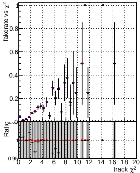
Fake rate vs. — DOM_V0001_R0000000001_Global_mkFit1000o_RECO — DOM_V0001_R0000000001_Global_mkFit1000o_RECO — DOM_V0001_R0000000001_Global_mkFit1000oTime_RECO
