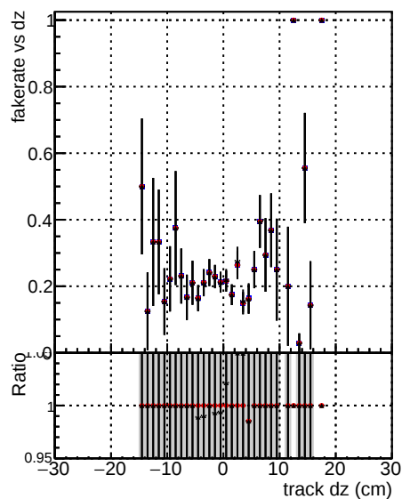
Fake rate vs dz DOM V0001 RECO DOM V0001 RECO Global mkFit10000 RECO Global mkFit10000 RECO Global mkFit10000 RECO
