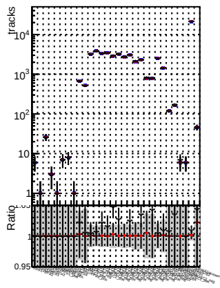
N of reco track vs. \chi^2 DQM V0001 R0000000001 Global mkFit1000 RECO DQM V0001 R0000000001 Global mkFit1000 RECO DQM V0001 R0000000001 Global mkFit1000 ATTime RECO
