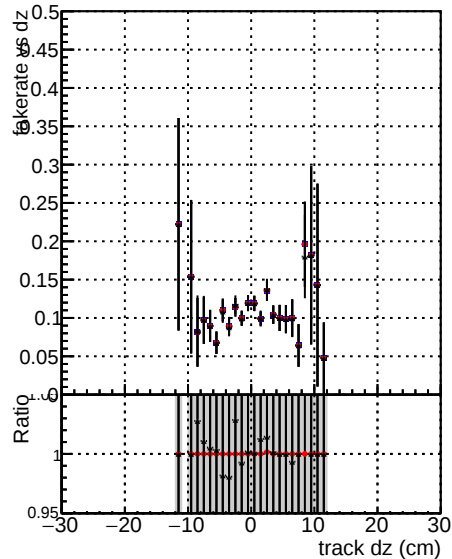
— DOM V0001 R0000000001 Global mkFit10000 RECO — DOM V0001 R0000000001 Global mkFit1000 RECO — DOM V0001 R0000000001 Global mkFit1000ATime RECO
