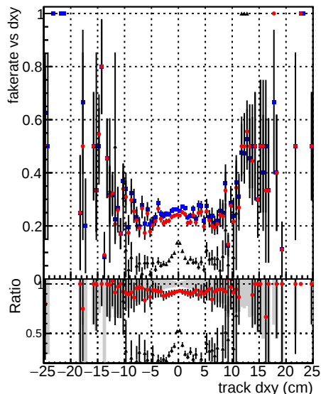
Legend for Fake rate vs dxy, Duplicates Rate vs Dxy, and Pileup rate vs dxy: DOM V0001 RECO (blue squares) DOM V0001 RECO (red circles) Global fit10000 RECO (black crosses) Global fit10000 RECO (black crosses) Global fit10000 RECO (black crosses)
