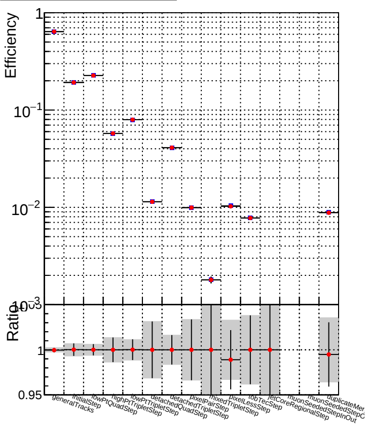
DQM_V0001_R0000000001_Global_mkFit1000o_RECO DQM_V0001_R0000000001_Global_mkFit1000_RECO
