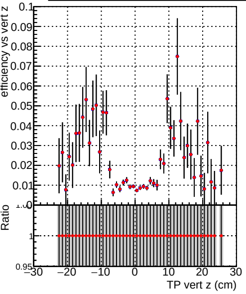
Efficiency vs vertpos Legend: DQM_V0001_R000000001_Global_mkFit1000o_RECO DQM_V0001_R000000001_Global_mkFit1000_RECO
