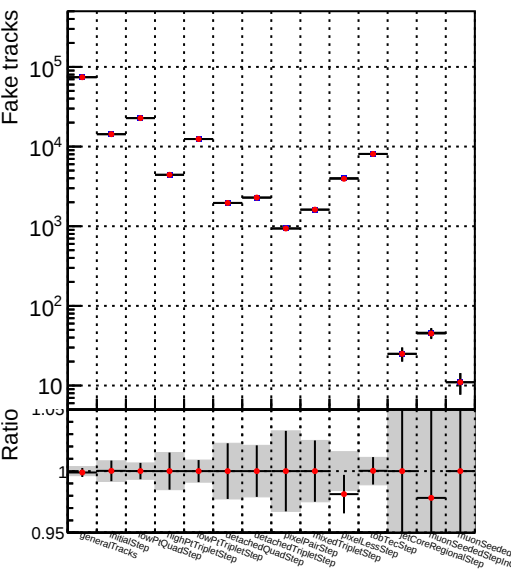
Number —● DQM_V0001_R000000001_Global_mkFit1000_RECO
