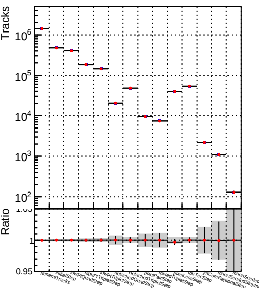
■ DQM_V0001_R0000000001_Global_mkFit1000o_RECO
