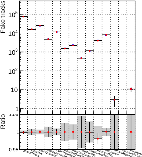
Number DQM_V0001_R000000001_Global_mkFit1000_RECO
