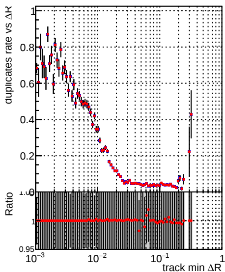
—●— DQM_V0001_R000000001_Global_mkFit1000o_RECO —●— DQM_V0001_R000000001_Global_mkFit1000_RECO
