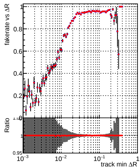
—●— DQM_V0001_R000000001_Global_mkFit1000o_RECO —●— DQM_V0001_R000000001_Global_mkFit1000_RECO
