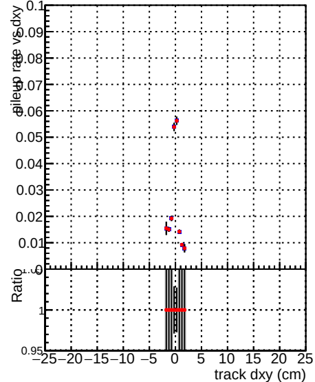
Global mkFit1000 RECO
