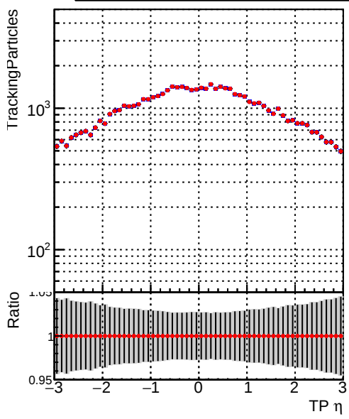
— DQM_V0001_R000000001_Global_mkFit1000o_RECO — DQM_V0001_R000000001_Global_mkFit1000_RECO
