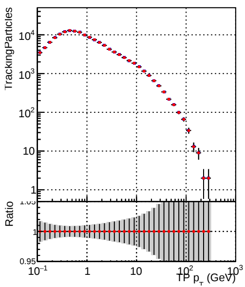
— DQM_V0001_R000000001_Global_mkFit1000o_RECO — DQM_V0001_R000000001_Global_mkFit1000_RECO
