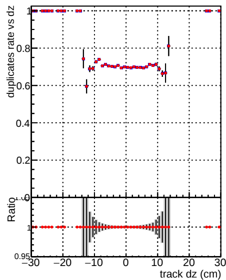
—●— DQM_V0001_R0000000001_Global_mkFit1000o_RECO —●— DQM_V0001_R0000000001_Global_mkFit1000_RECO
