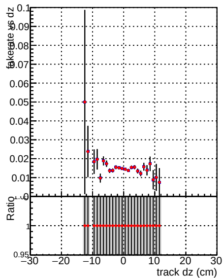
DQM V0001_R0000000001 Global mkFit1000o RECO Fake rate vs dz Duplicates Rate vs Dxy Pileup rate vs dxy Fake rate vs dz Duplicates Rate vs Dxy Pileup rate vs dxy
