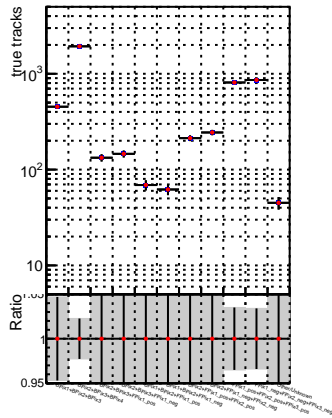
Global_mkFit1000o_RECO Global_mkFit1000o_RECO
