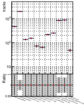
Global_mkFit1000o_RECO Global_mkFit1000o_RECO
