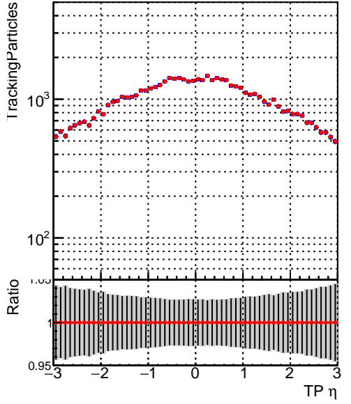
■ DQM_V0001_R000000001_Global_mkFit1000o_RECO ◆ DQM_V0001_R000000001_Global_mkFit1000o_RECO
