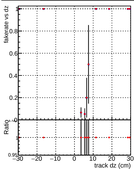
Fake rate vs dz Global mkFit1000o RECO DQM_V0001_R0000000001 Global mkFit1000 RECO DQM_V0001_R0000000001
