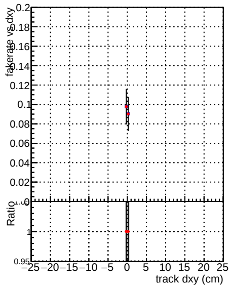
Global mkFit1000o RECO Fake rate vs d █ █ █ Duplicates Rate vs Dxy █ █ █ Pileup rate vs dxy █ █ █
