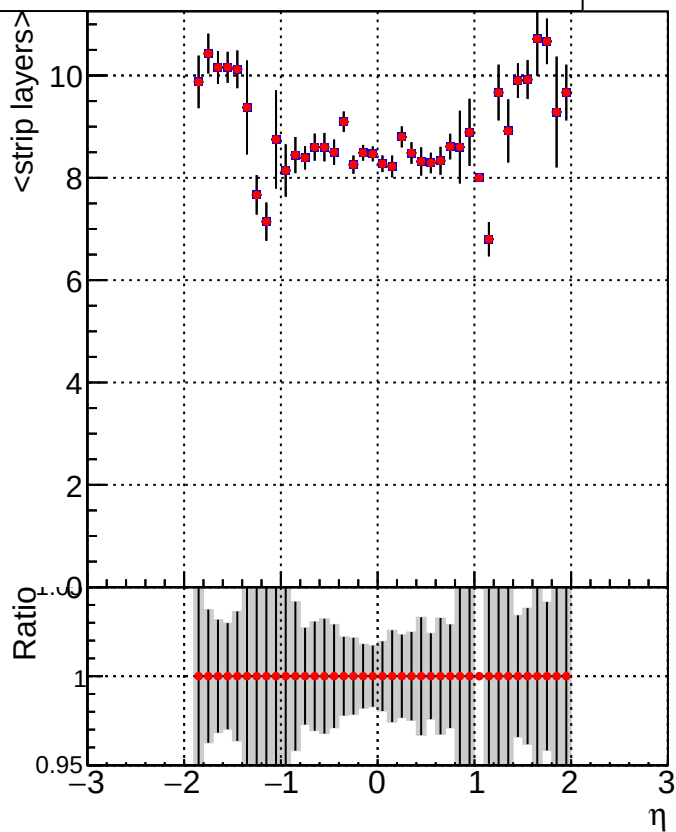
Legend: DQM_V0001_R0000000001_Global_mkFit1000o_RECO DQM_V0001_R0000000001_Global_mkFit1000_RECO
