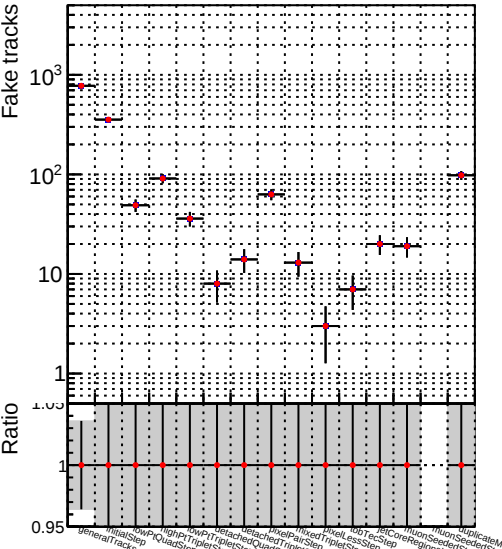
Number ● DQM_V0001_R000000001_Global_mkFit1000_RECO
