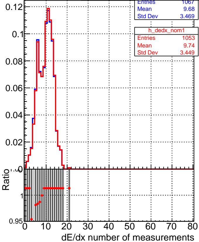
■ DQM_V0001_R000000001_Global_mkFit1000o_RECO ● DQM_V0001_R000000001_Global_mkFit1000_RECO
