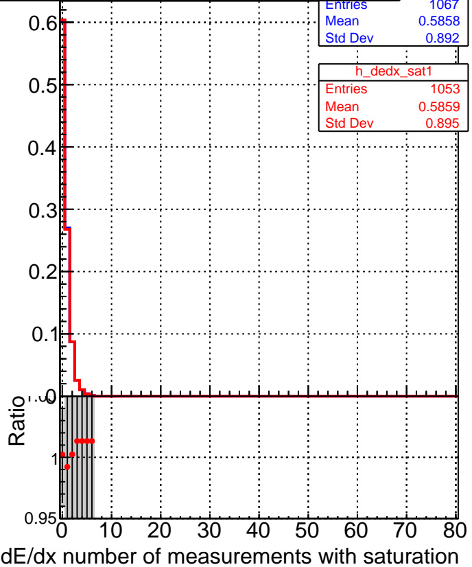
■ DQM_V0001_R000000001_Global_mkFit1000o_RECO ● DQM_V0001_R000000001_Global_mkFit1000_RECO
