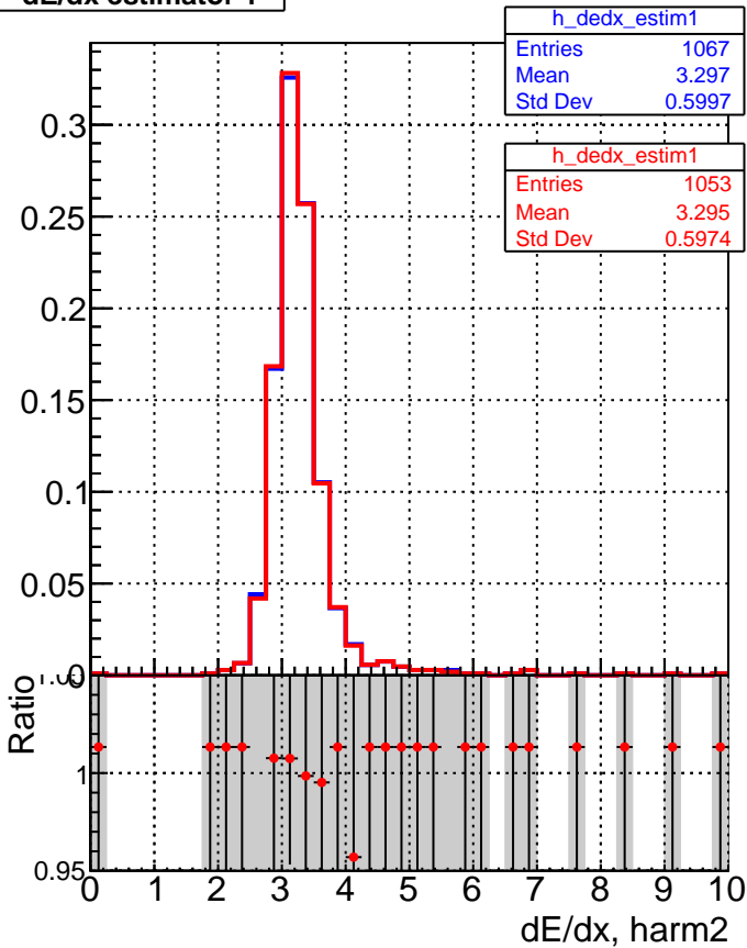
■ DQM_V0001_R000000001_Global_mkFit1000o_RECO ● DQM_V0001_R000000001_Global_mkFit1000_RECO
