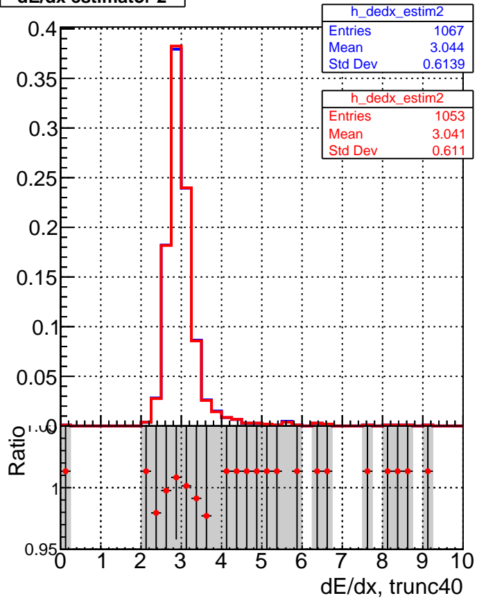
■ DQM_V0001_R000000001_Global_mkFit1000o_RECO ● DQM_V0001_R000000001_Global_mkFit1000_RECO
