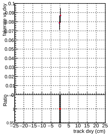
—●— DQM_V0001_R0000000001_Global_mkFit1000o_RECO —●— DQM_V0001_R0000000001_Global_mkFit1000_RECO
