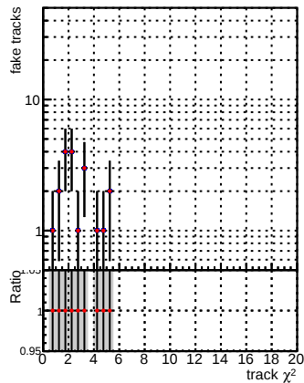
Legend: - Global_mkFit1000o_RECO (black line) - DQM_V0001_R000000001 (red line) - Global_mkFit1000o_RECO (black line) - DQM_V0001_R000000001 (red line)
