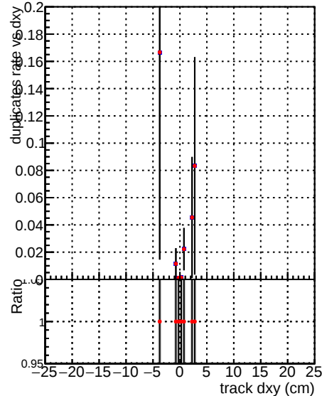
al_mkFit1000_RECO
