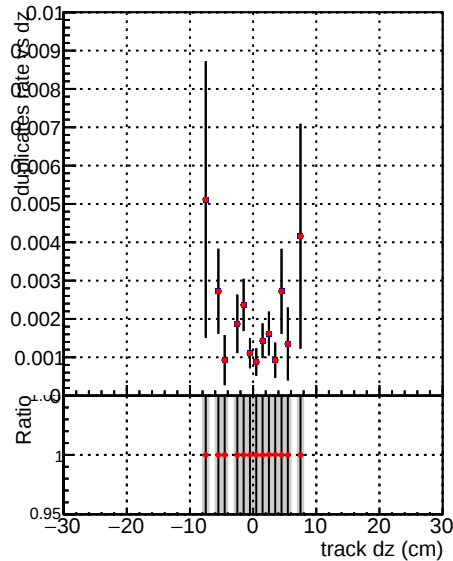
al_mkFit1000_RECO
