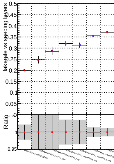
Fake rate vs. Legend Global mkFit1000o RECO Grey line with error bars DQM_V0001_R0000000001 Global mkFit1000o Red line with error bars DQM_V0001_R0000000001 Global mkFit1000o
